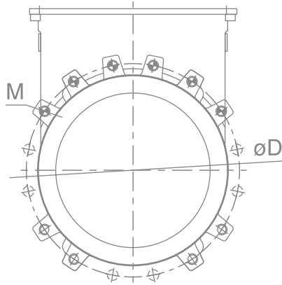
NPS 18
